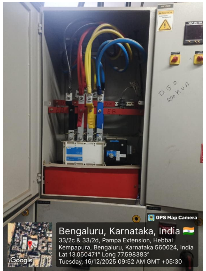
Generator Changeover
